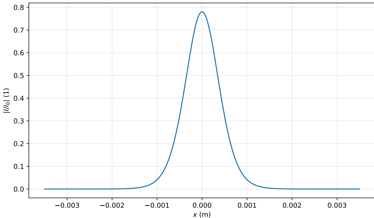
Intensity profile I(x, y = 0, z = 2.149m)/I_0 , P_{in}=0.5P_{cr} , artificial time
